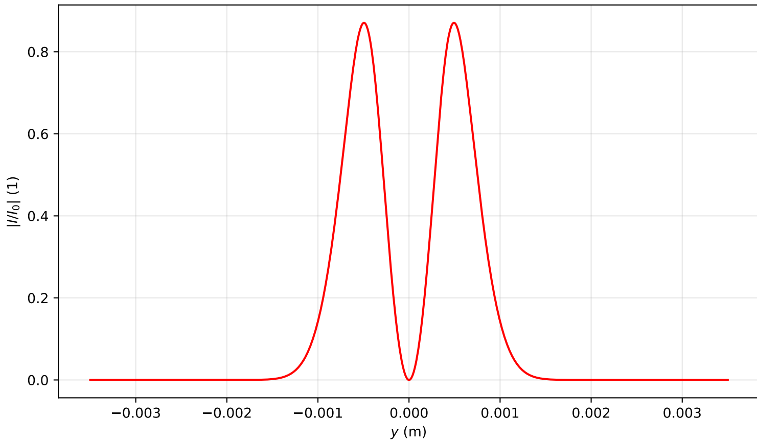
Intensity profile I(x=0, y, z=0.159)/I_0 , P_{in}=5.0P_{cr} , artificial time
